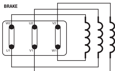
Connection Δ (minimum rated voltage)
