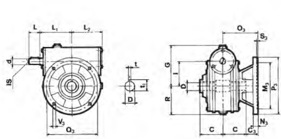
I... FBR VERSION
