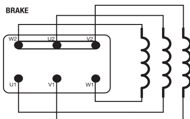
Connection Δ (maximum rated voltage)
